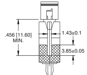
DETAIL C-C
