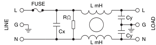
CIRCUIT DIAGRAM
