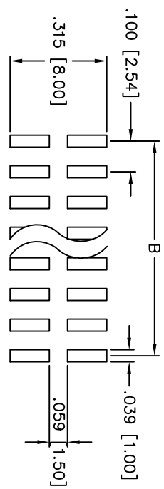
Recommended P.C.B Layout
