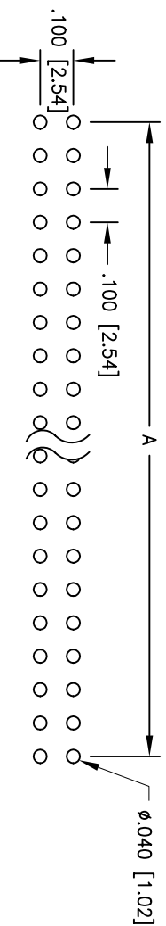
PCB LAYOUT
