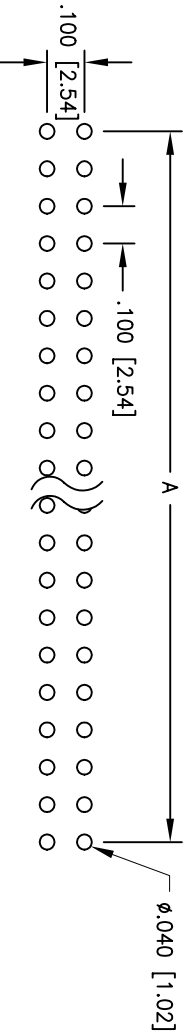
PCB LAYOUT
