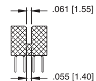
DETAIL B-B
