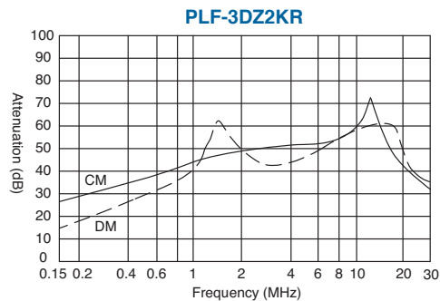
Insertion Loss in dB (Measured in 50 \Omega systems, as IEC / cispr No. 17)
