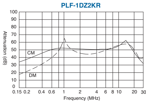
Insertion Loss in dB (Measured in 50 \Omega systems, as IEC / cispr No. 17)
