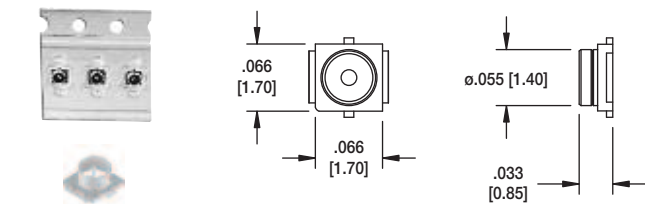
RF28-01-T-00-50-G Enlarged to show detail
