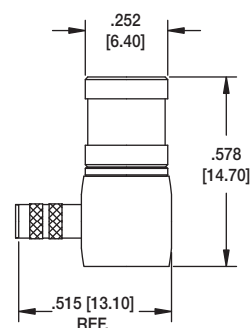
RF3 TYPE 03 SMB MALE RIGHT ANGLE CRIMP
