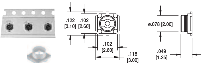
RF20-01-P-00-50-G Enlarged to show detail
