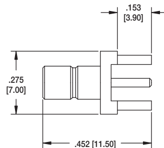
RF3 TYPE 05 SMB FEMALE PCB MOUNT
