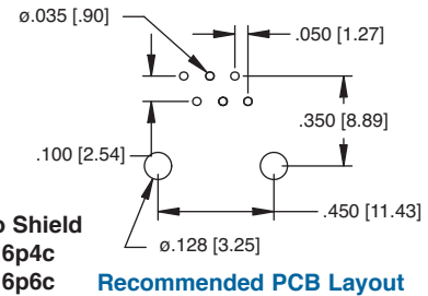
MTJ-88MX1-FSE-PG Metal Shielded with panel ground tabs
